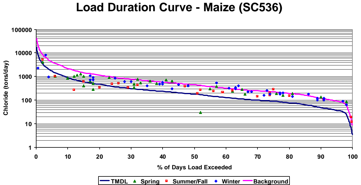
Figure 2. Load Curve – Maize
