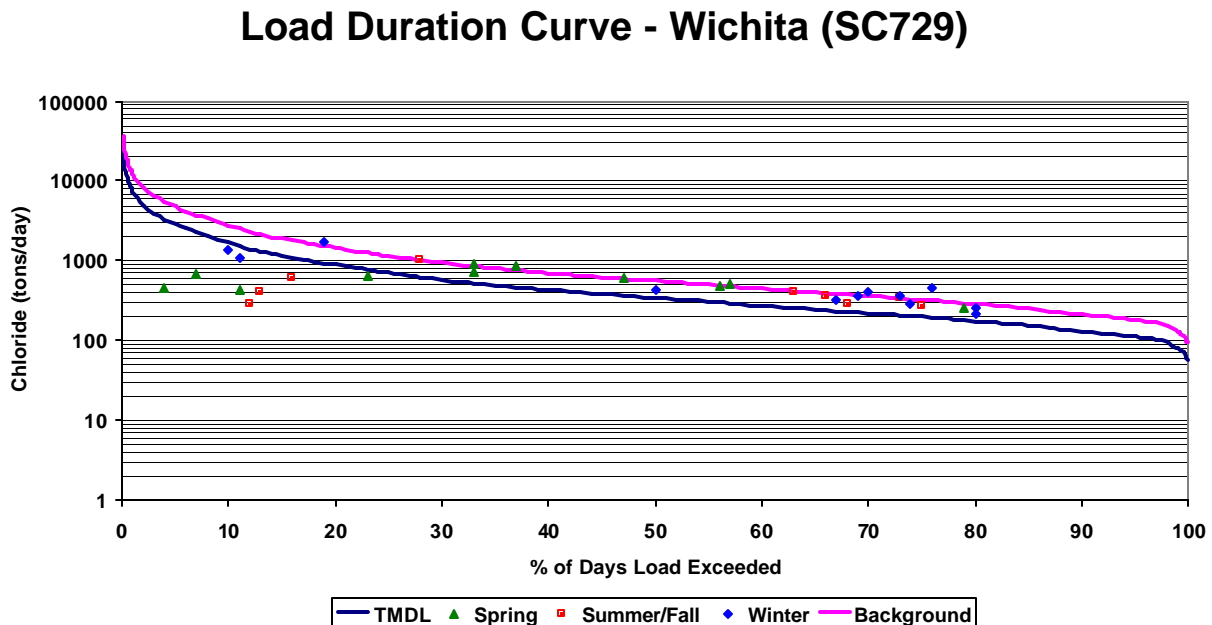
Figure 3. Load Curve – Wichita
